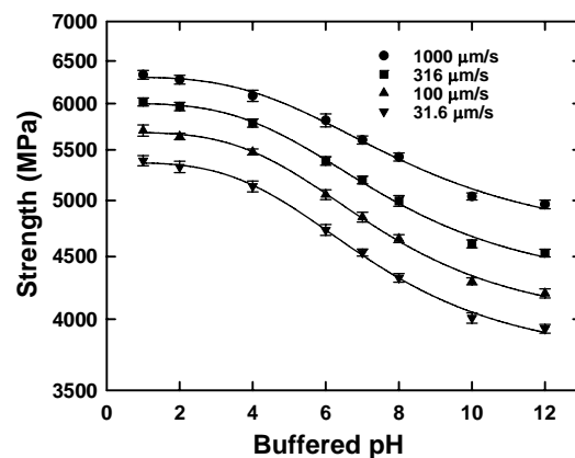
Figure 2. Strength of bare fiber in two-point bending at 4 loading rates in various 25°C pH buffer solutions.
