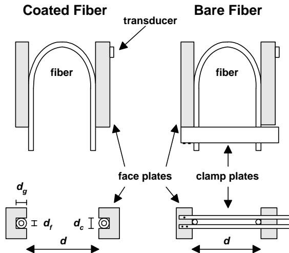
Figure 1. Two-point bending apparatus for bare and coated optical fiber.
