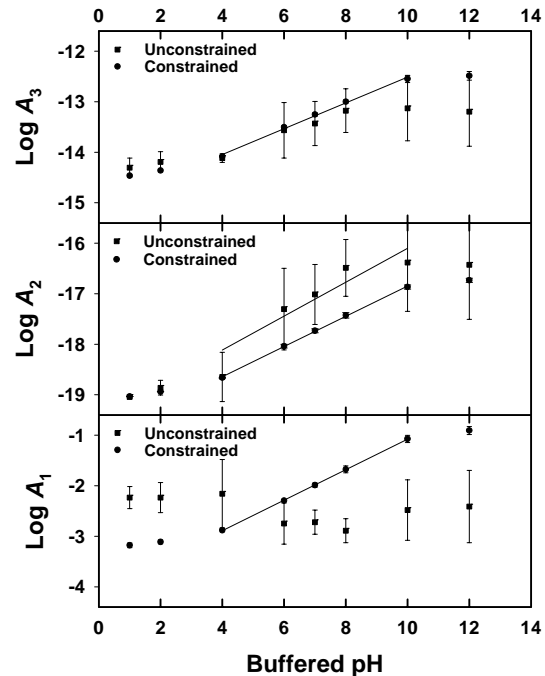
Figure 8. \log A_i vs. pH for models 1, 2, and 3 for bare fiber at 25°C showing both as fitted and constrained values.
