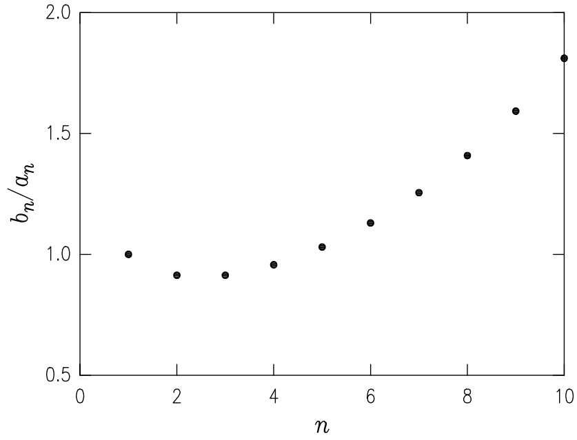
Figure 3. Ratio of the power series coefficients in two-point bending and mandrel bending as a function of coefficient order, n .
