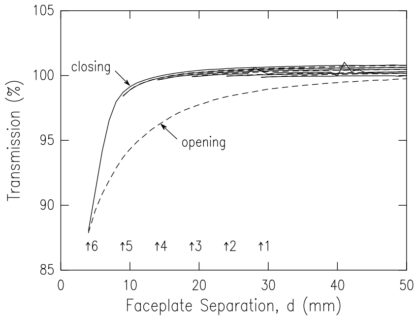
Figure 2. Optical transmission as a function of faceplate separation for a 250 \mu\text{m} plastic fiber in two-point bending. Results are shown for six successive closings and openings.
