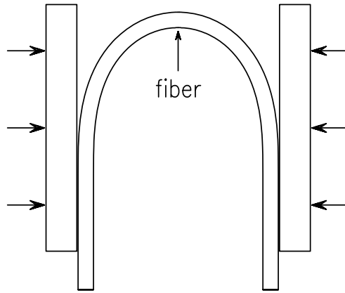
Figure 1. Schematic of the two-point bend technique for fiber optical loss, strength and fatigue measurement.
