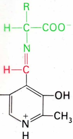
Aldimine
