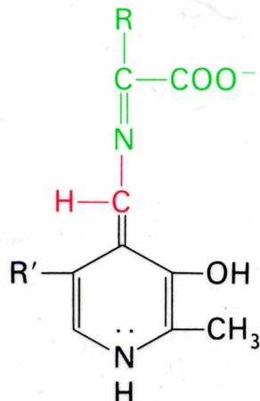
Quinonoid intermediate
