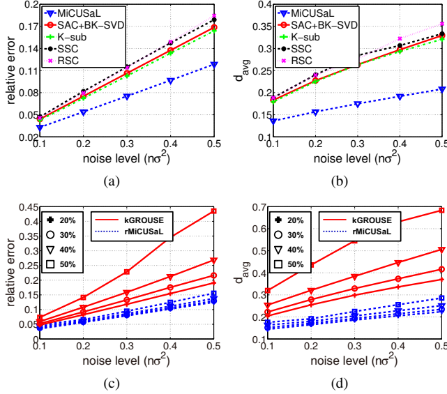
Fig. 1. Comparison of MC-UoS learning performance on synthetic data. (a) and (b) show relative errors and d_{avg} 's for complete data. (c) and (d) show relative errors and d_{avg} 's for missing data case.
